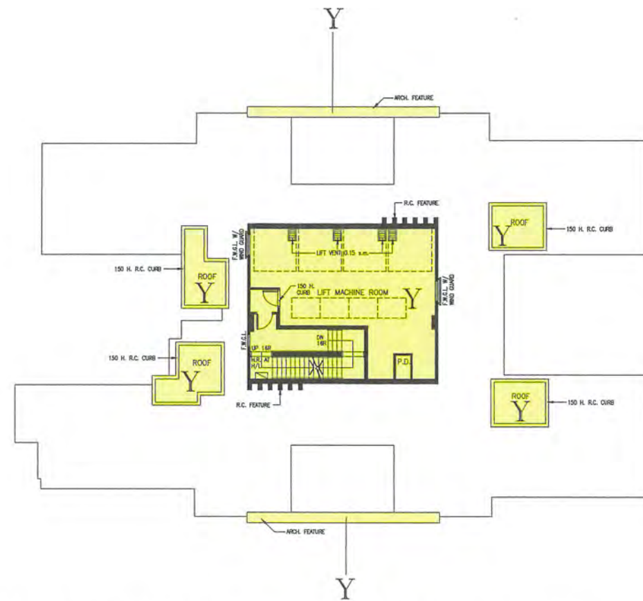
LIFT MACHINE ROOM LEVEL PLAN
