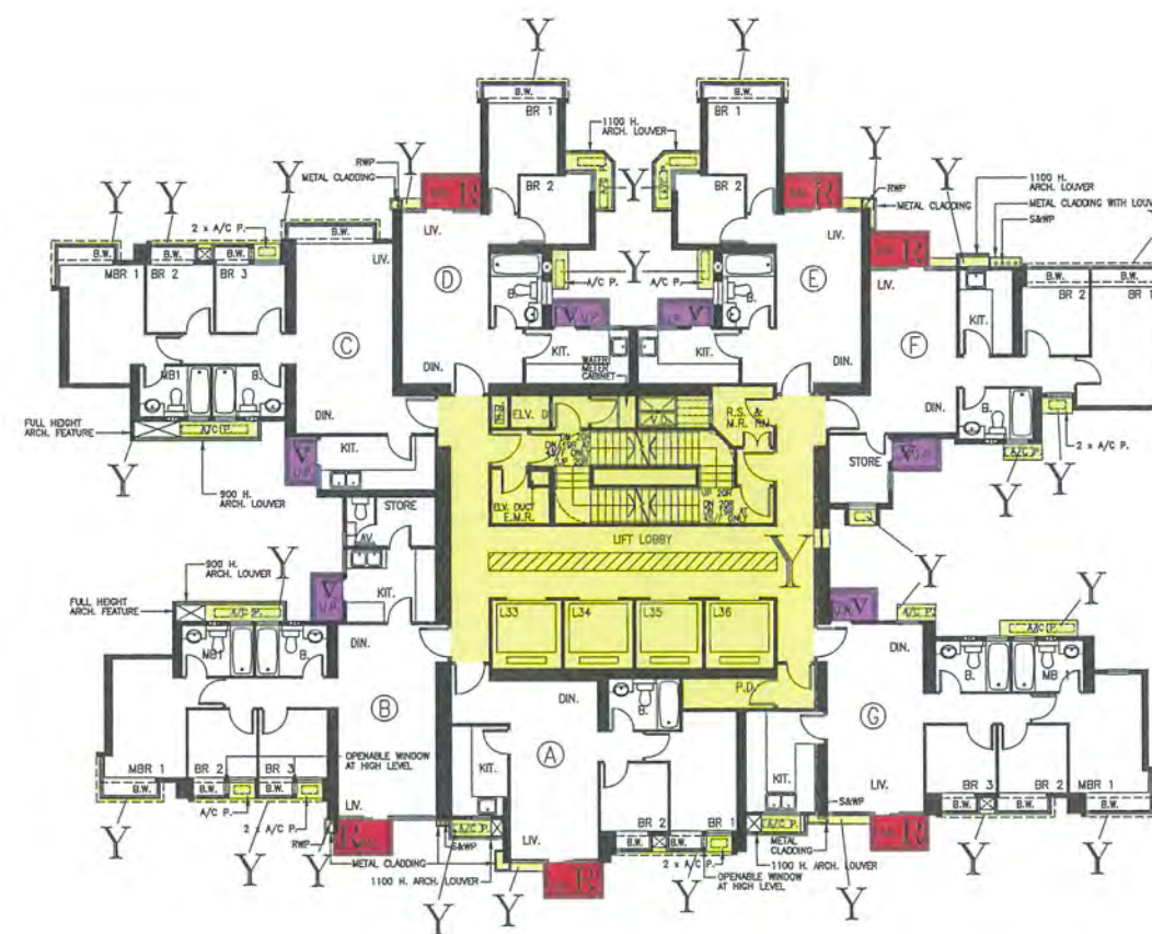
45th-48th FLOOR PLAN
