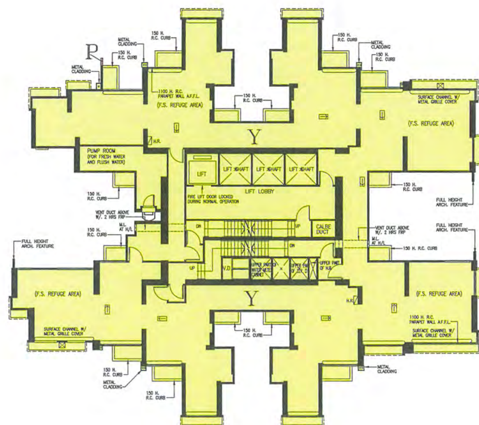
23rd REFUGE FLOOR PLAN
