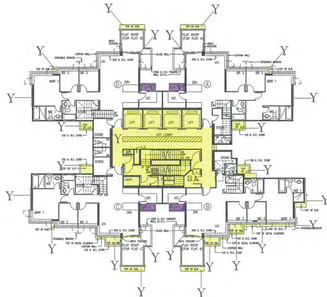
43rd FLOOR PLAN
