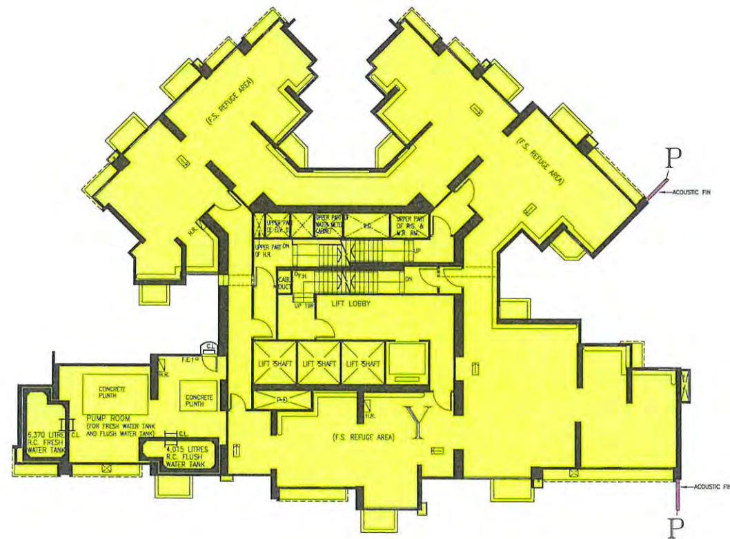
23rd REFUGE FLOOR PLAN
