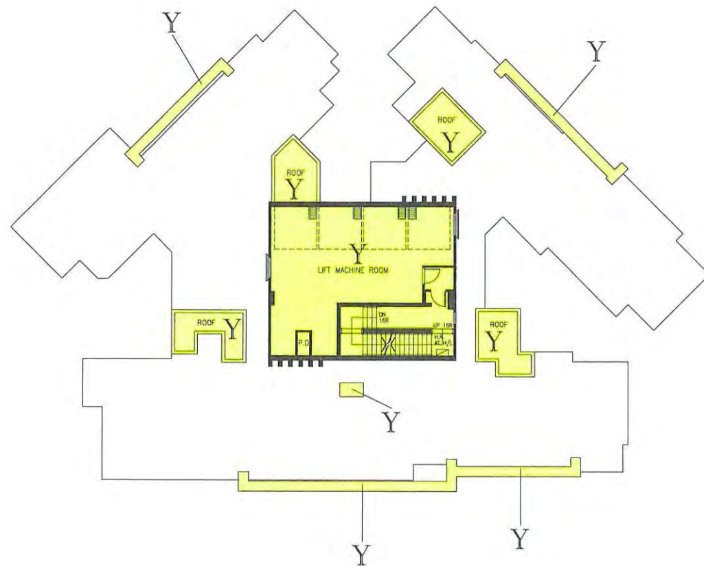
LIFT MACHINE ROOM LEVEL PLAN
