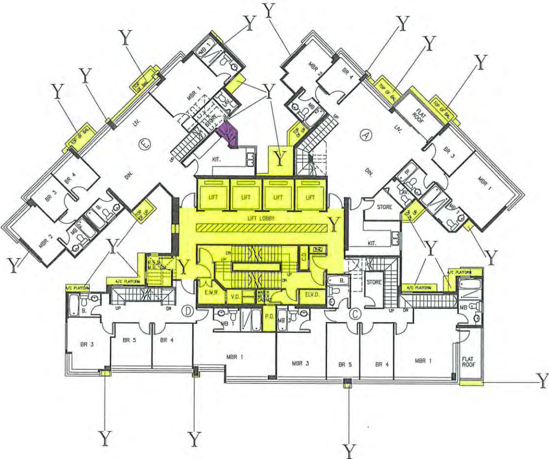
50th FLOOR PLAN
