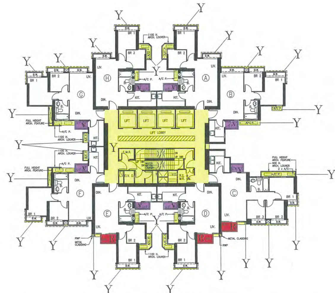
25th TO 40th FLOOR PLAN
