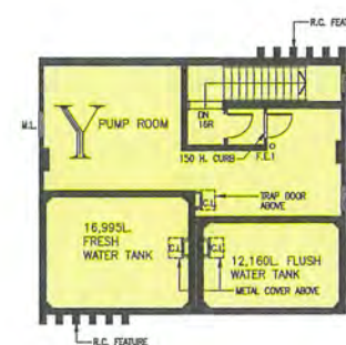
WATER TANK LEVEL
