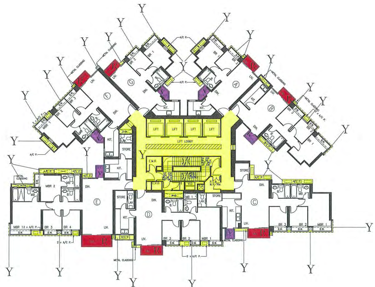
46th & 47th FLOOR PLAN
