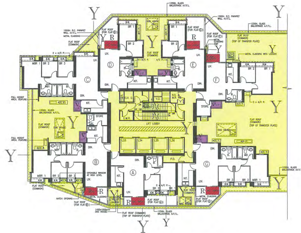
6th FLOOR PLAN
