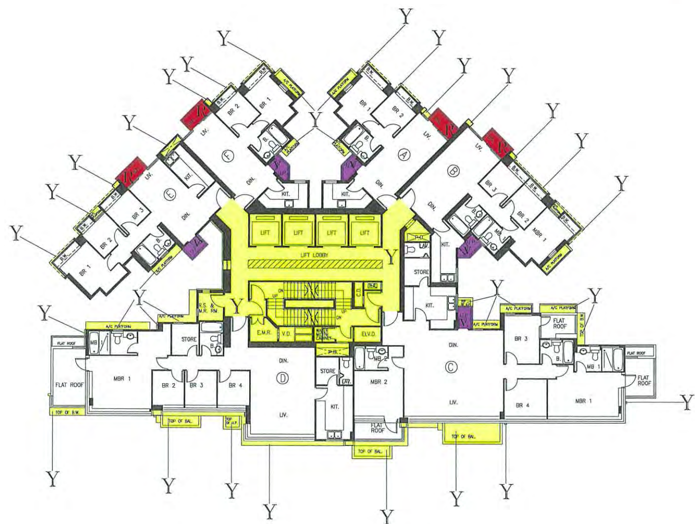
48th FLOOR PLAN
