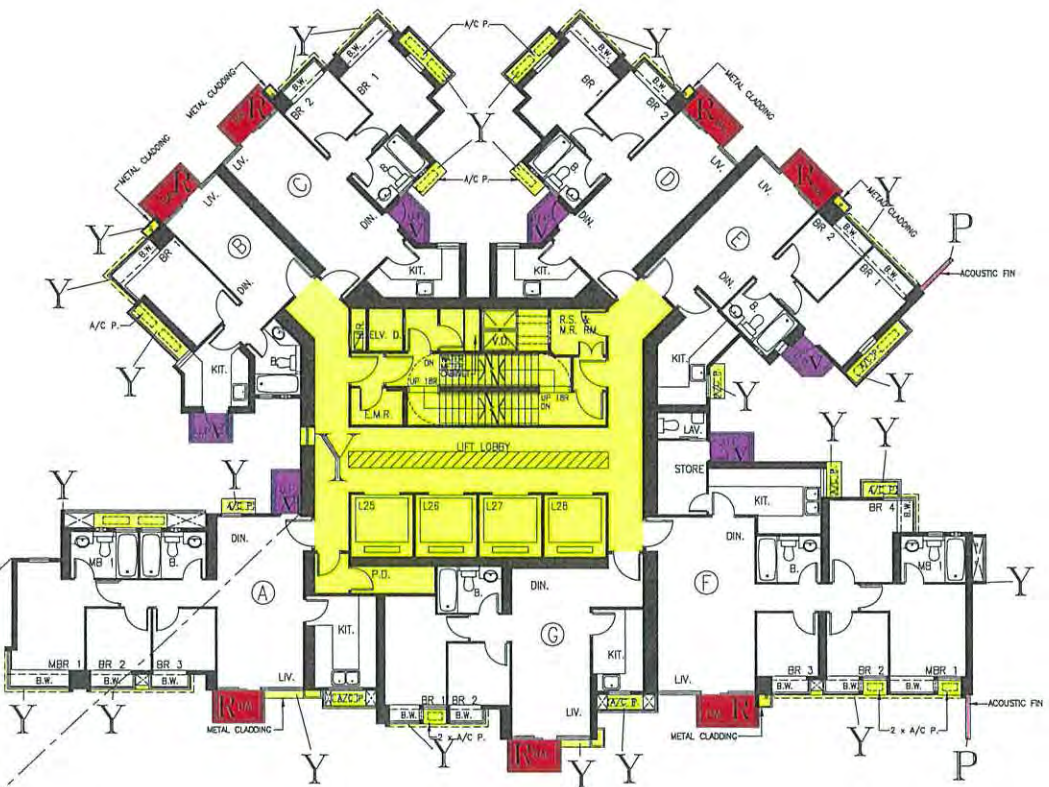
7th-22nd FLOOR PLAN
