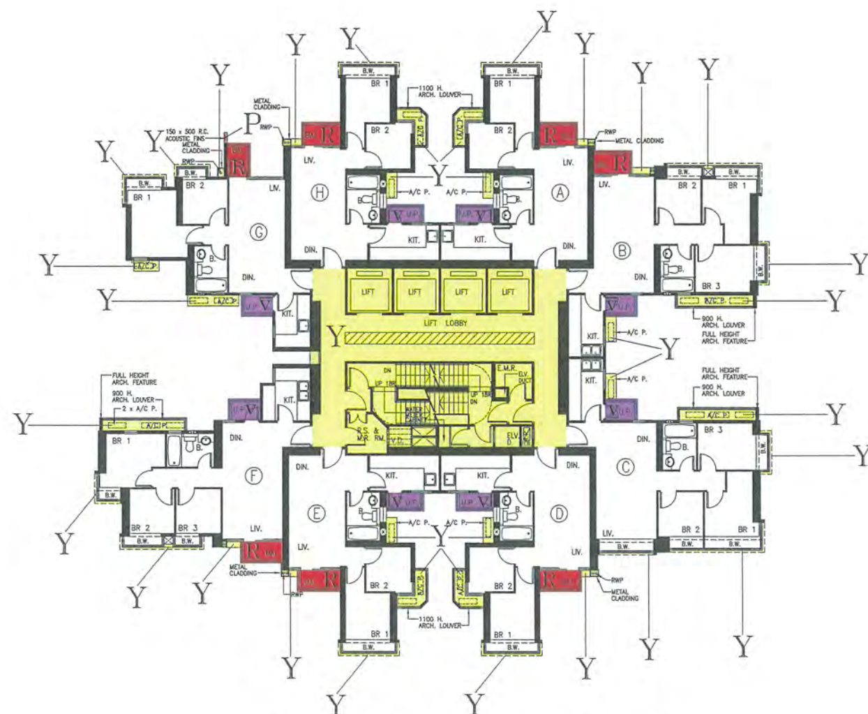
46th FLOOR PLAN
