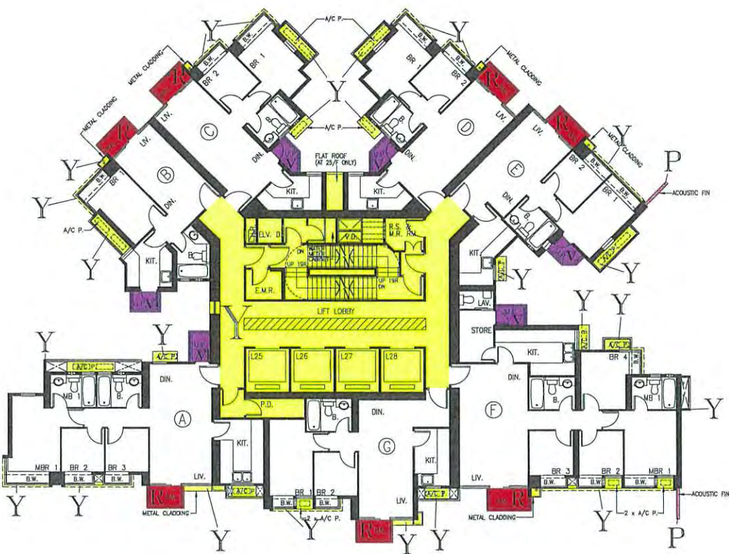
25th-42nd FLOOR PLAN
