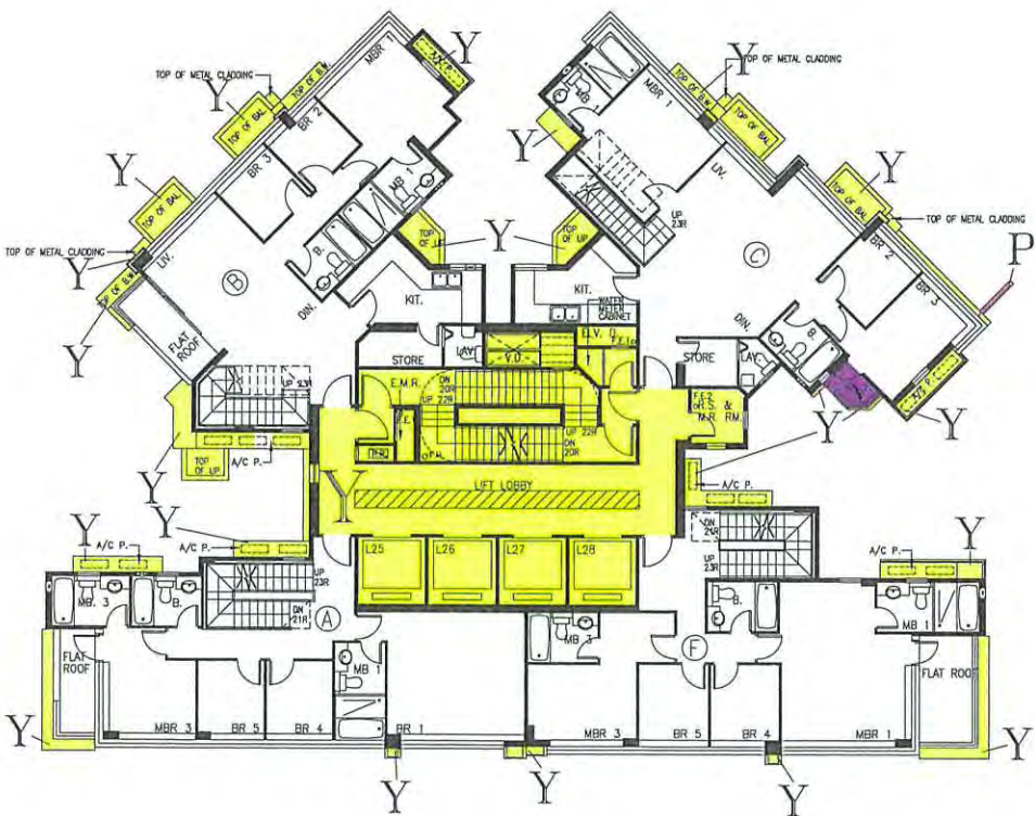
51st FLOOR PLAN
