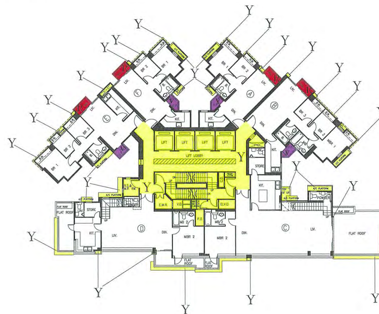
49th FLOOR PLAN
