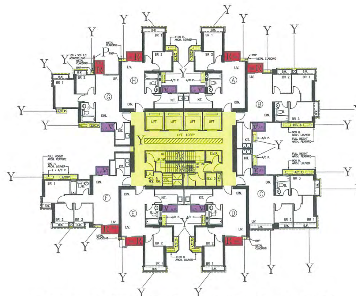
25th TO 45th FLOOR PLAN
