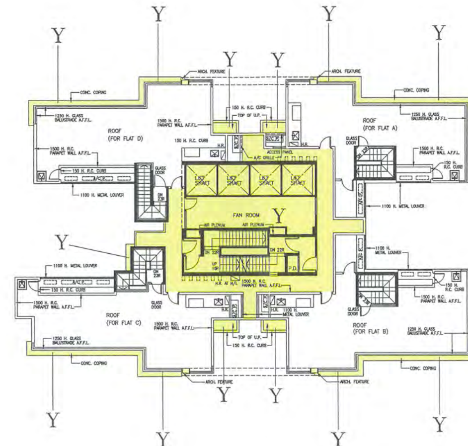
ROOF PLAN
