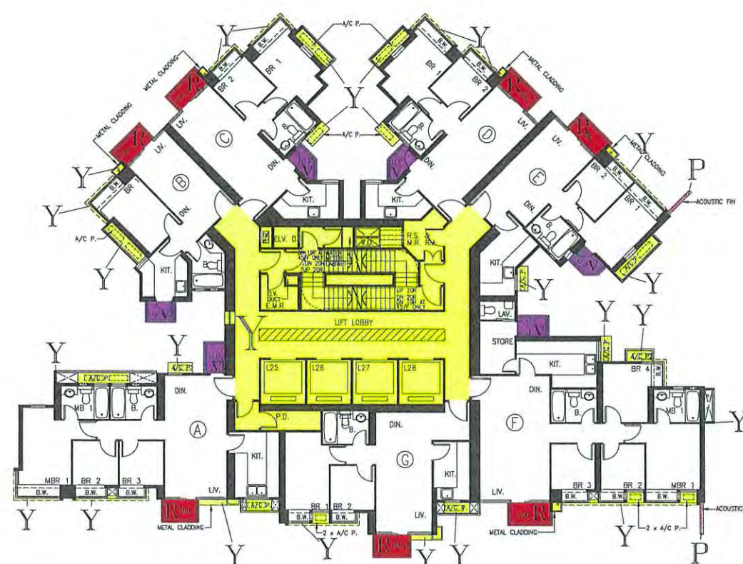
45th-48th FLOOR PLAN
