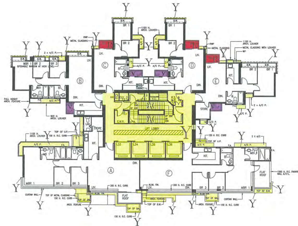
49th FLOOR PLAN
