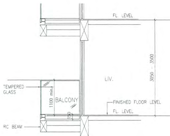
2 TYPICAL SECTION THRU. BALCONY SCALE 1 : 40
