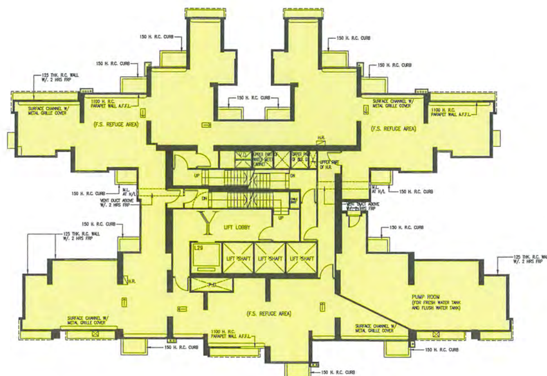
23rd REFUGE FLOOR PLAN
