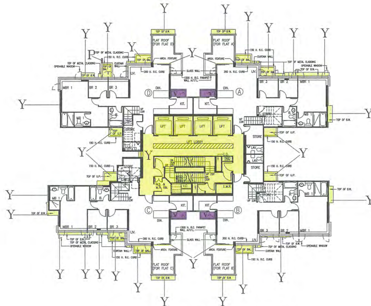
48th FLOOR PLAN
