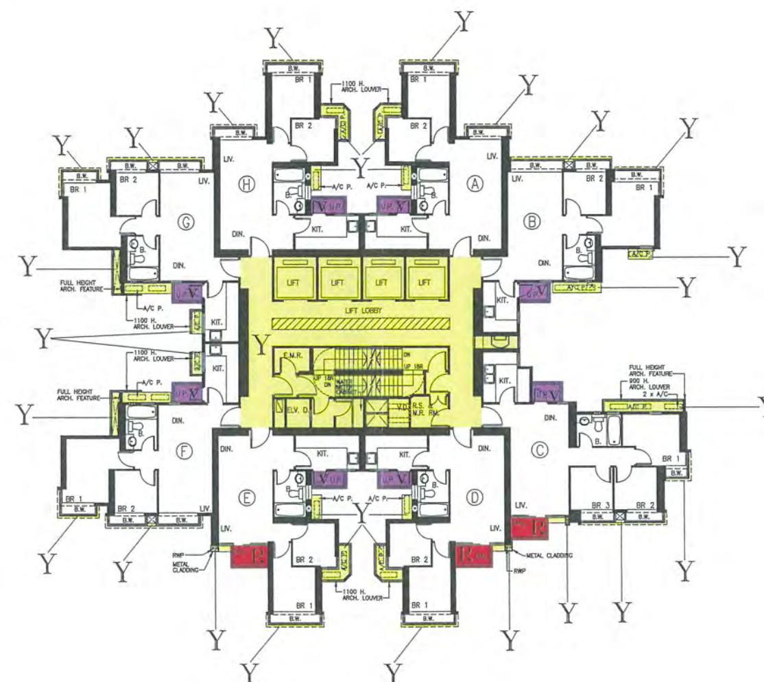
7th TO 22nd FLOOR PLAN
