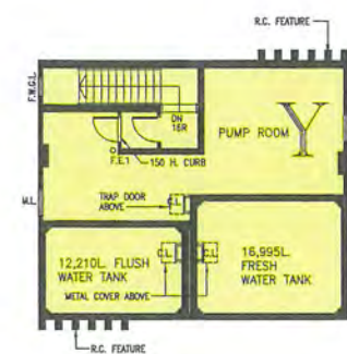
WATER TANK LEVEL
