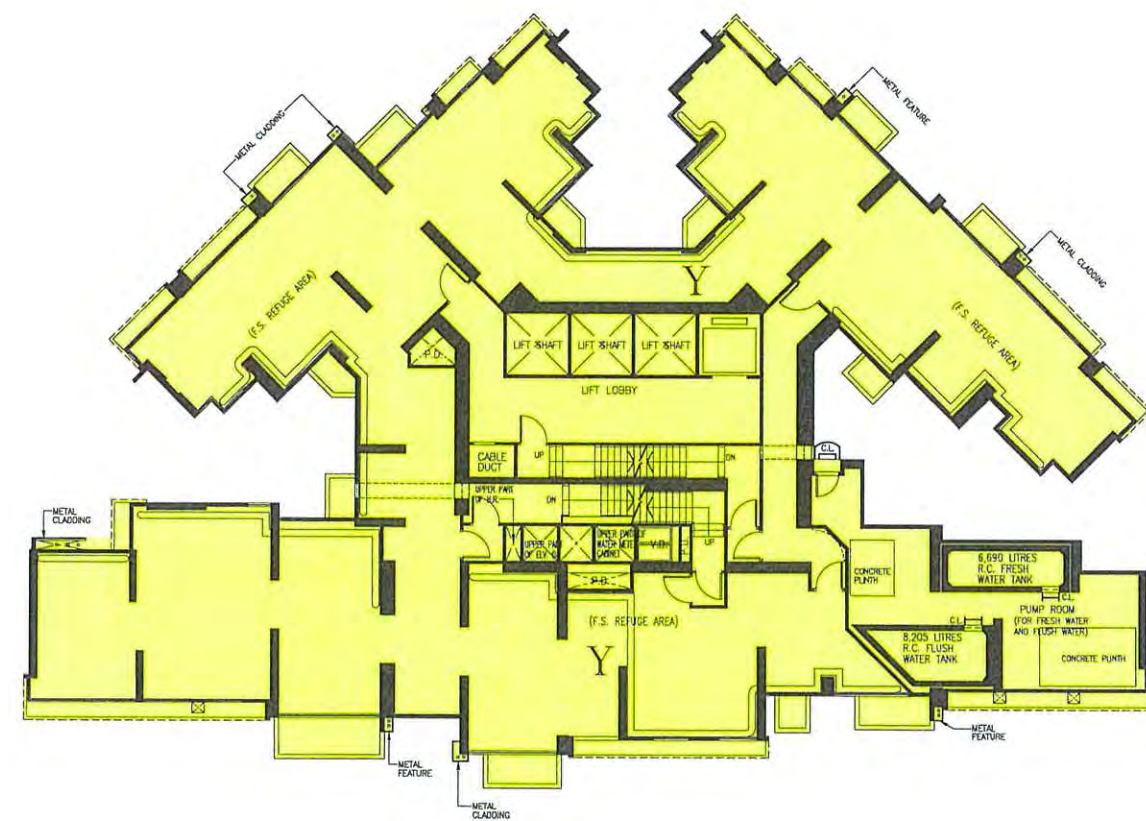
23rd REFUGE FLOOR PLAN
