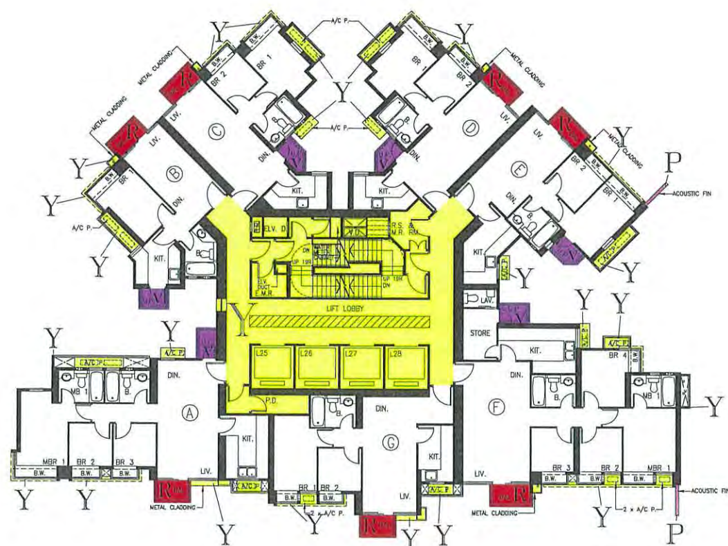
43rd FLOOR PLAN
