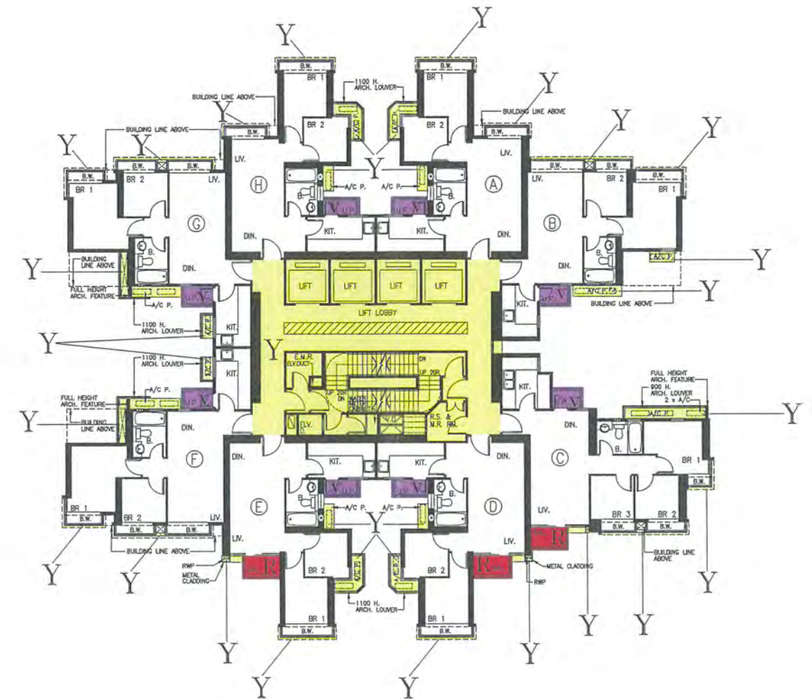
42nd FLOOR PLAN
