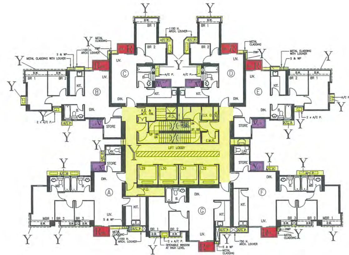
7th-22nd FLOOR PLAN
