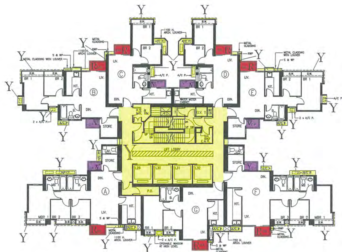
43rd FLOOR PLAN
