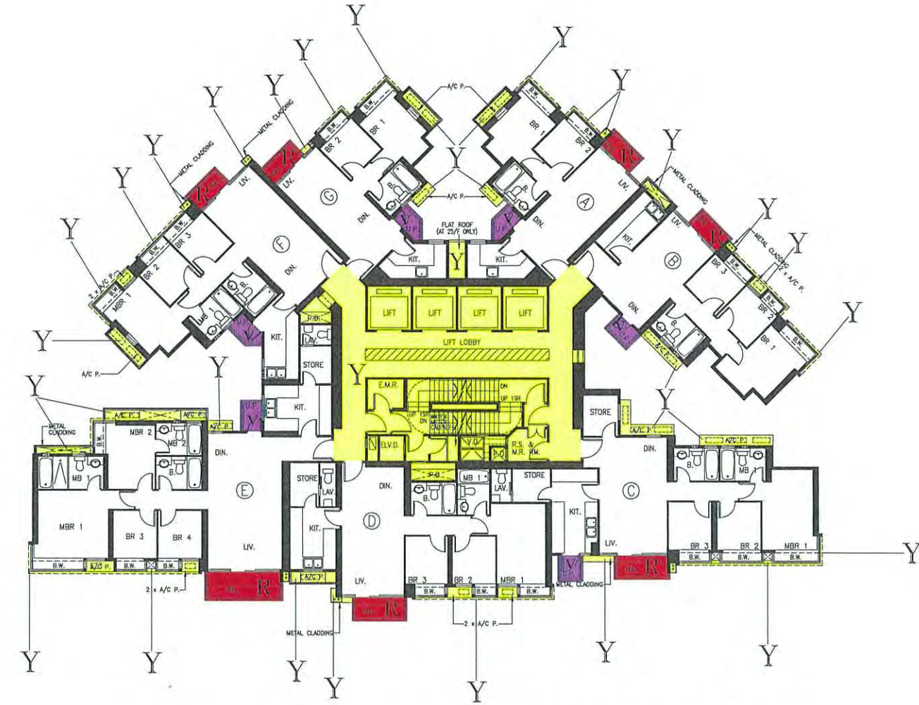
25th TO 43rd FLOOR PLAN
