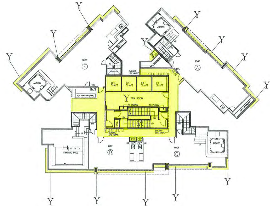
ROOF PLAN
