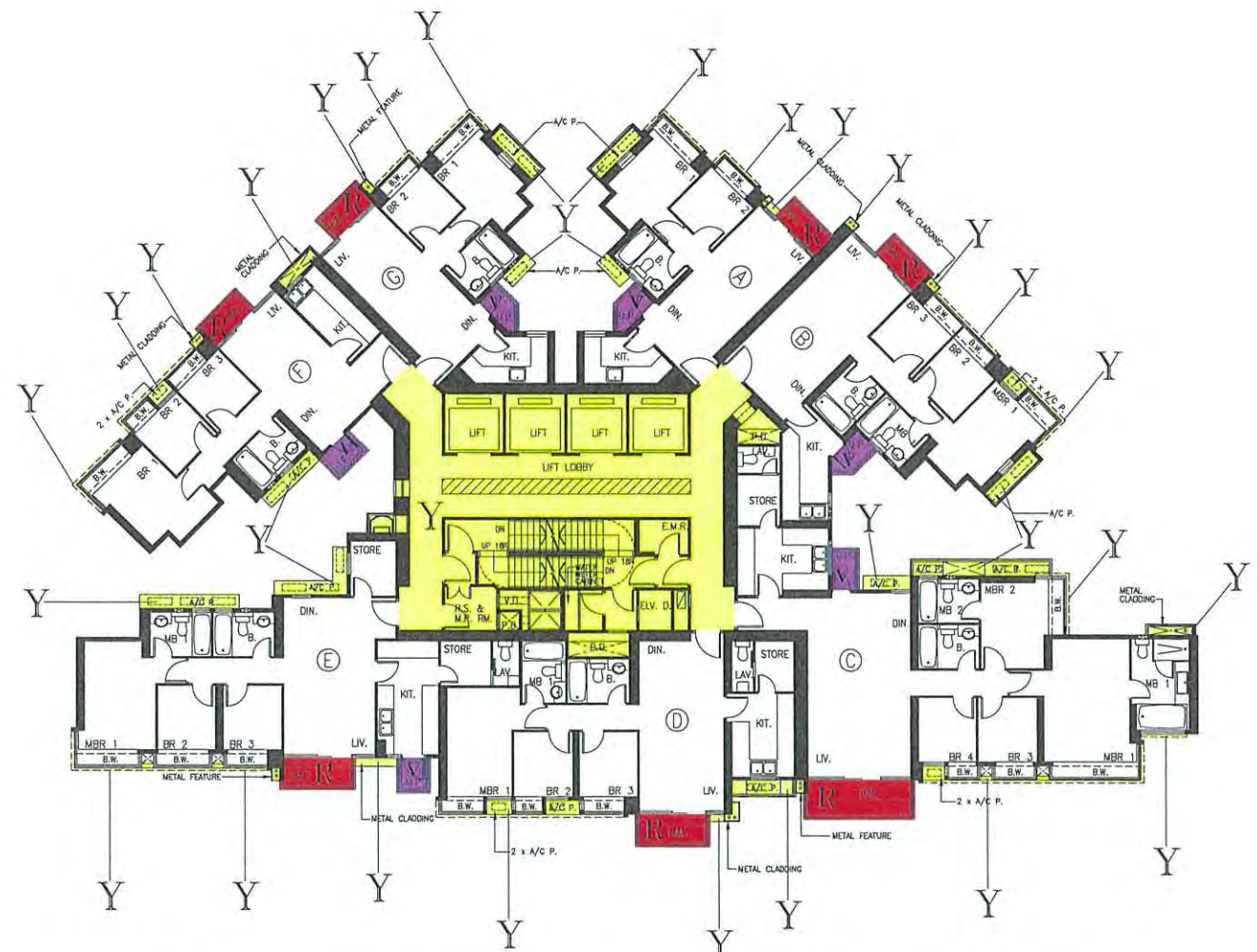
7th TO 22nd FLOOR PLAN
