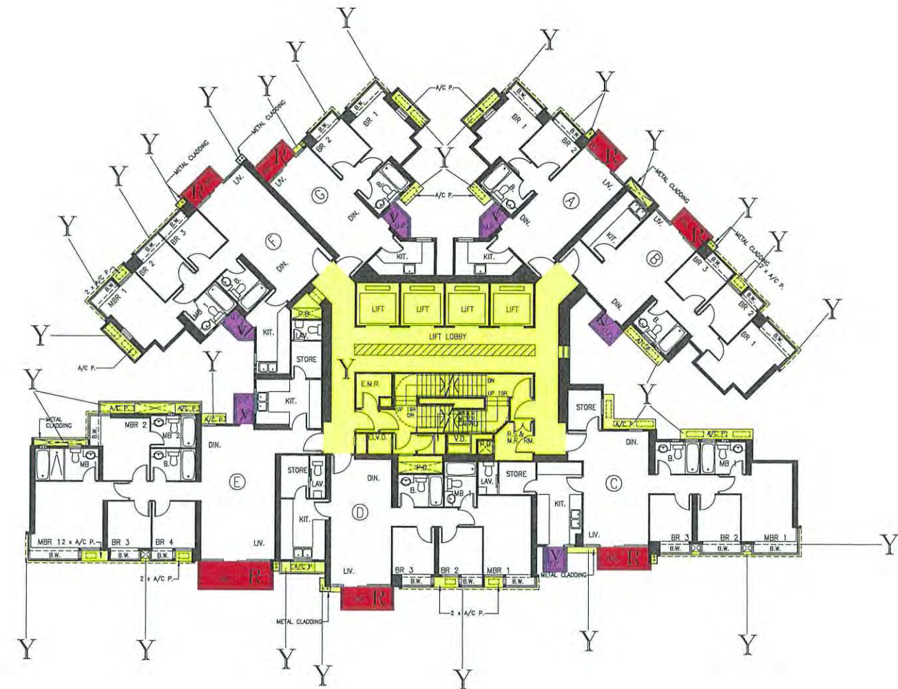
45th FLOOR PLAN
