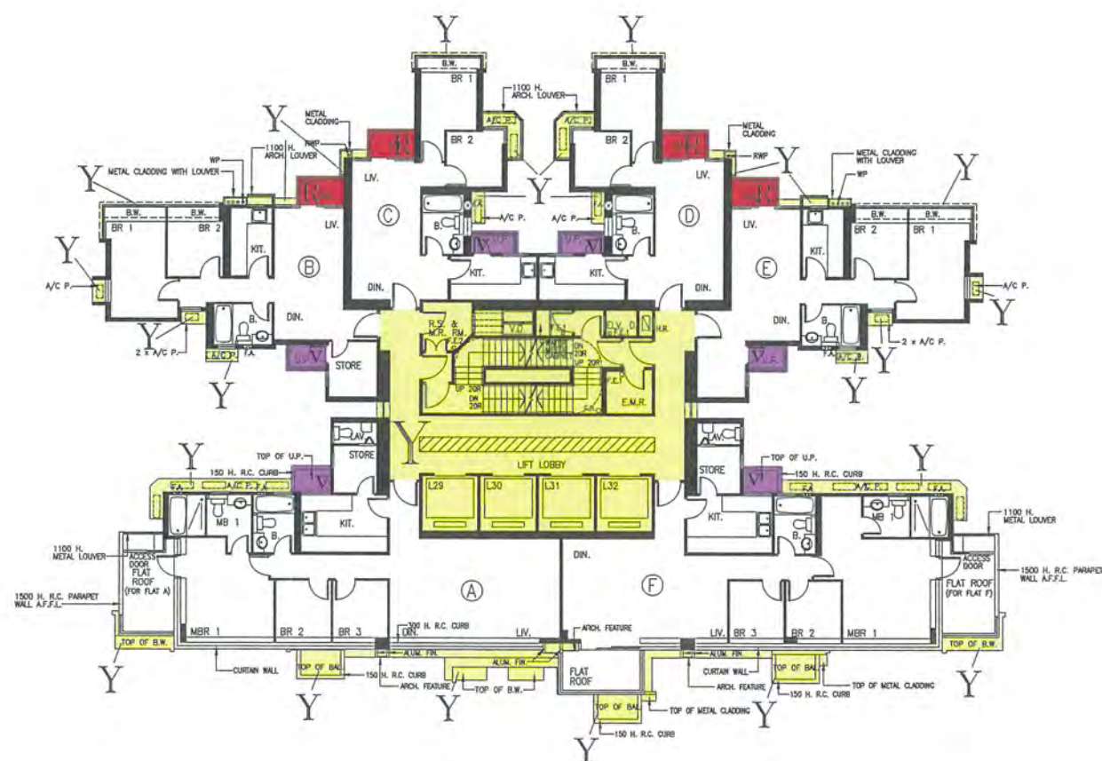
49th FLOOR PLAN
