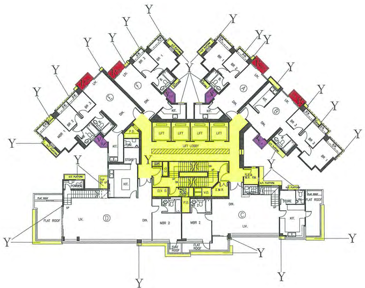
49th FLOOR PLAN
