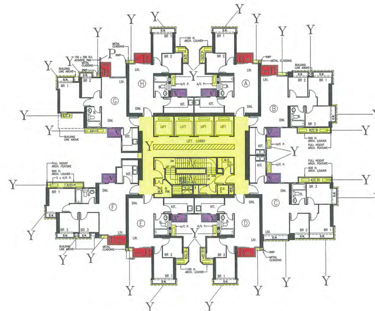
47th FLOOR PLAN
