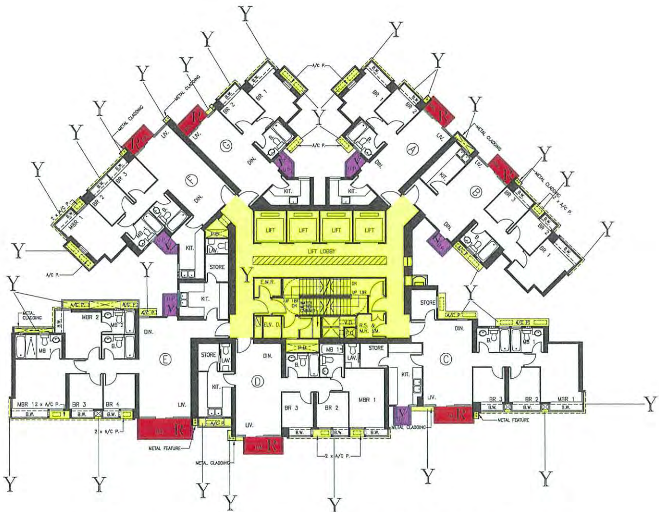
7th TO 22nd FLOOR PLAN
